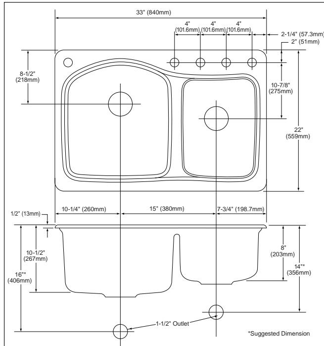
FSW420GS.5 Bridgeport Self-rimming Cast Iron Kitchen Sink
